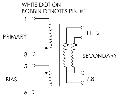
FIGURE 1: SCHEMATIC DIAGRAM
